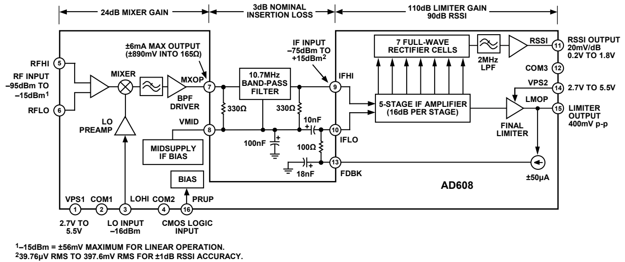
Figure 22. Functional Block Diagram
